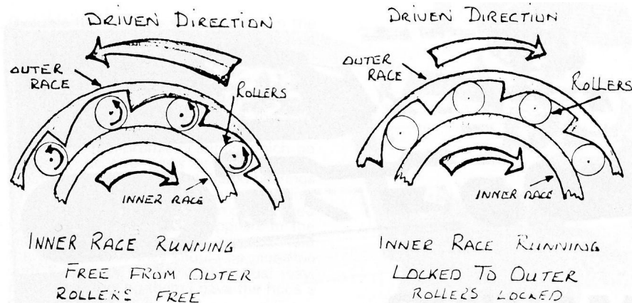
Sketch 2 Roller Clutch.
